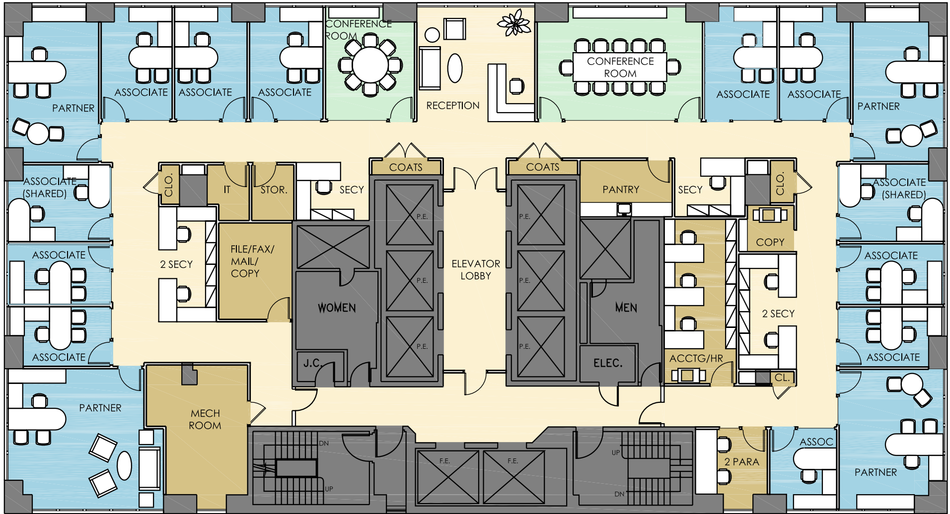
1 TYPICAL TOWER FLOOR PLAN
